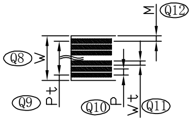
DETAIL OF TERMINAL
