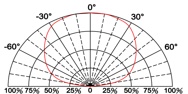
Fig.6 Directive Radiation
