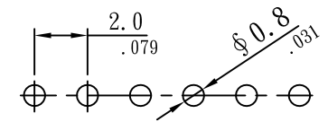
PCB LAYOUT
