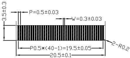
DETAIL "A" (S=3:1)
