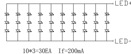
LED CIRCUIT DIAGRAM:
