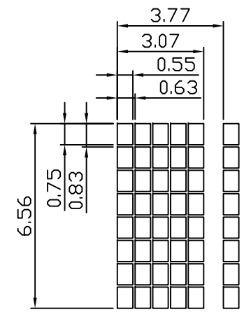
Display Pattern
