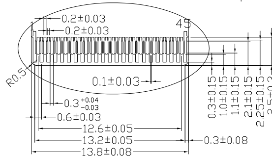
DETAIL A(3:1)
