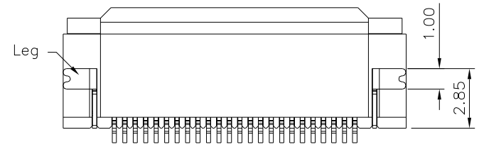
FPC Slot Dimension
