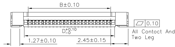
FPC Slot Dimension
