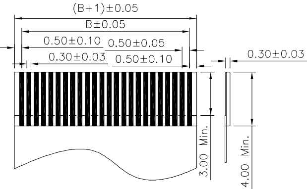
Recommended FPC Dimension
